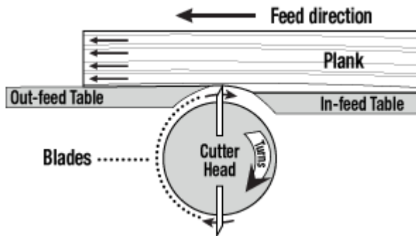
Figure 2 – Jointer
